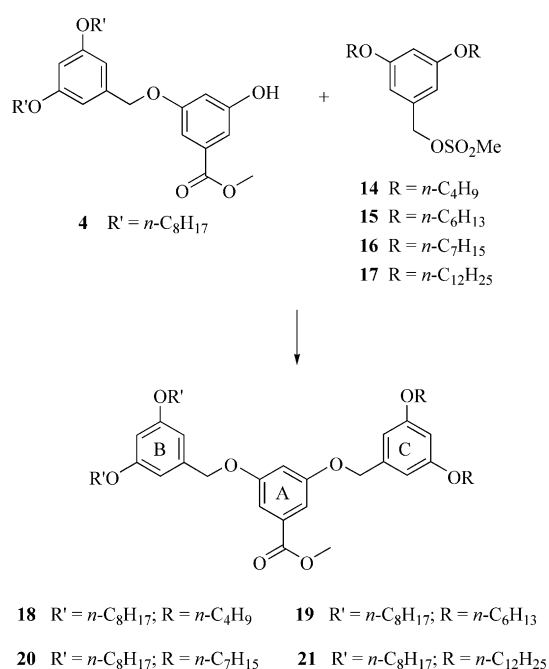
Scheme 5. Formation of asymmetrical alkyl-decorated Fréchet dendrons. Ring labels for NMR spectroscopic assignments.
