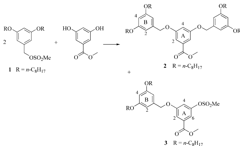
Scheme 2. Formation of a symmetrical octyl-decorated Fréchet dendron and the mesylate by-product used as a building block for the asymmetrical dendrons. Ring labels for NMR spectroscopic assignments.
