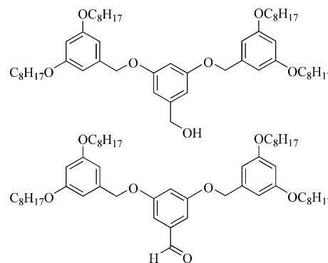
Scheme 1. Octyl-decorated second-generation Fréchet-type dendrons. [12,15]
