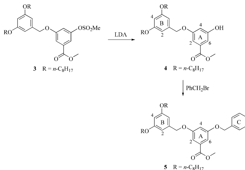
Scheme 3. Synthetic pathway to the asymmetrical dendron 5 . Ring labels for NMR spectroscopic assignments.
