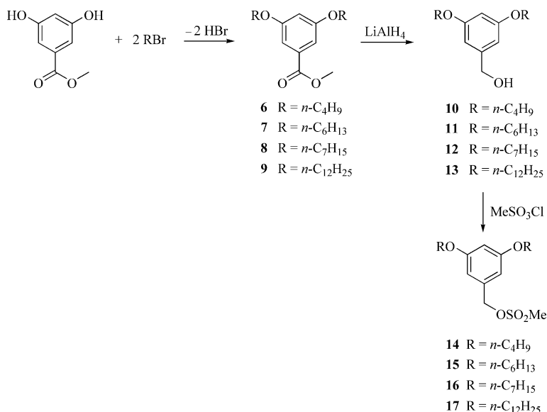
Scheme 4. Reaction scheme for the formation of mesylate building blocks.
